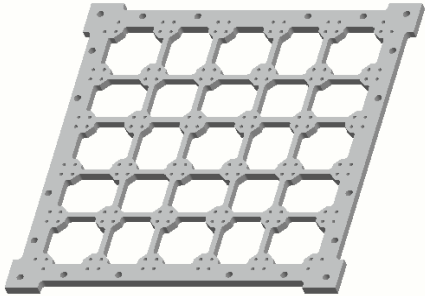
M-BA01A 5x5 Array Cell
