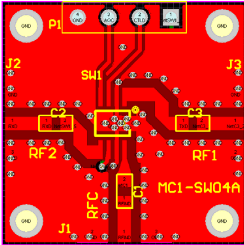
MC1-SW04A PCB Layout:
