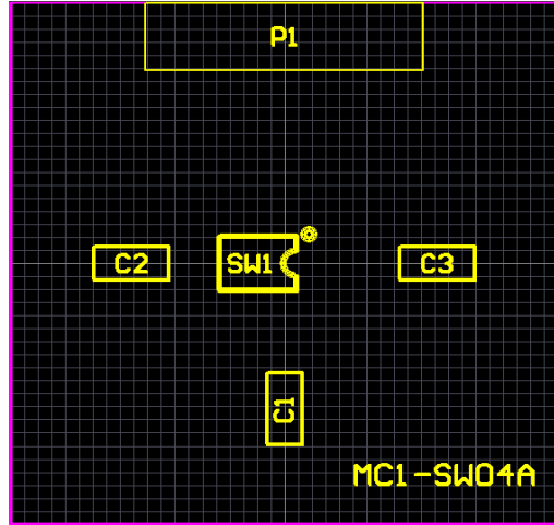
MC1-SW04A Assembly Drawing:
