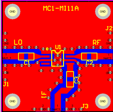
MC1-MI11A PCB Layout:
