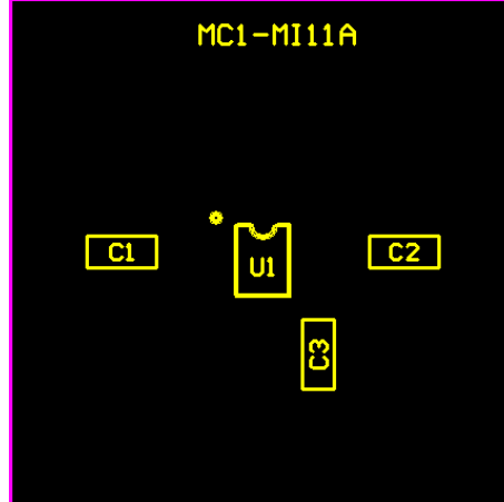
MC1-MI11A Assembly Drawing:
