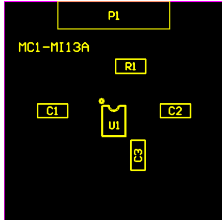
MC1-MI13A Assembly Drawing:
