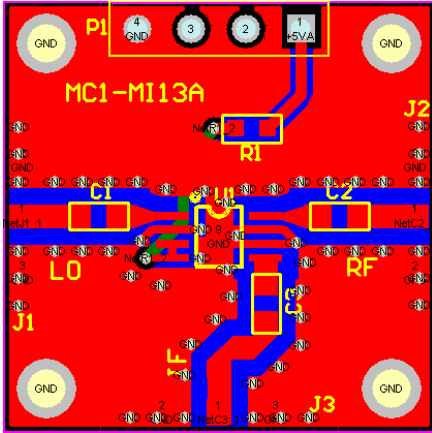
MC1-MI13A PCB Layout:
